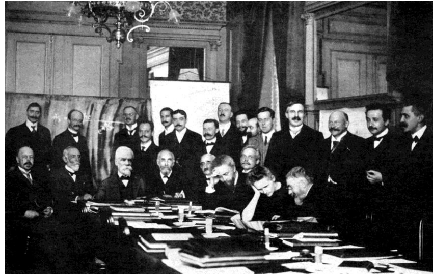
The first Solvay Conference (1911)
