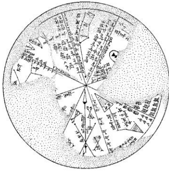
Assyrian star map from Nineve
