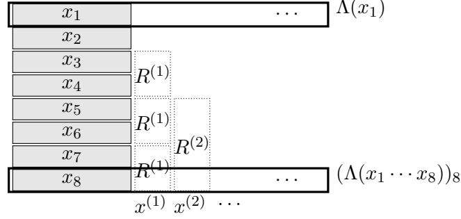
Figure 1: An illustration of the tree code's encoding.
