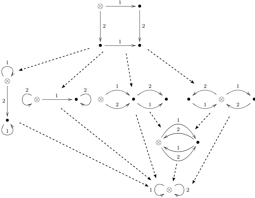
FIGURE 3.4. The subgraph of \mathcal{D}_k induced by [H, \infty)_{\overline{x}} , that is, all quotients of the core graph \Gamma = \Gamma_X(H) , for H = \langle x_1 x_2 x_1^{-1} x_2^{-1} \rangle . The dashed arrows denote immediate quotients, i.e. quotients generated by merging a single pair of vertices. \Gamma has exactly seven quotients: itself, four immediate quotients, and two quotients at distance 2.
