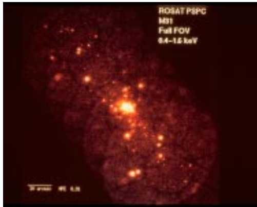
Fig. 3. A recent X-ray image of the Andromeda galaxy, M31. More than 5% of the sources lie in globular clusters belonging to Andromeda. Original colour image by courtesy of the ROSAT Mission ( http://www.xray.mpe.mpg.de/ ) and the Max-Planck-Institut für extraterrestrische Physik ( http://www.mpe.mpg.de/ )
