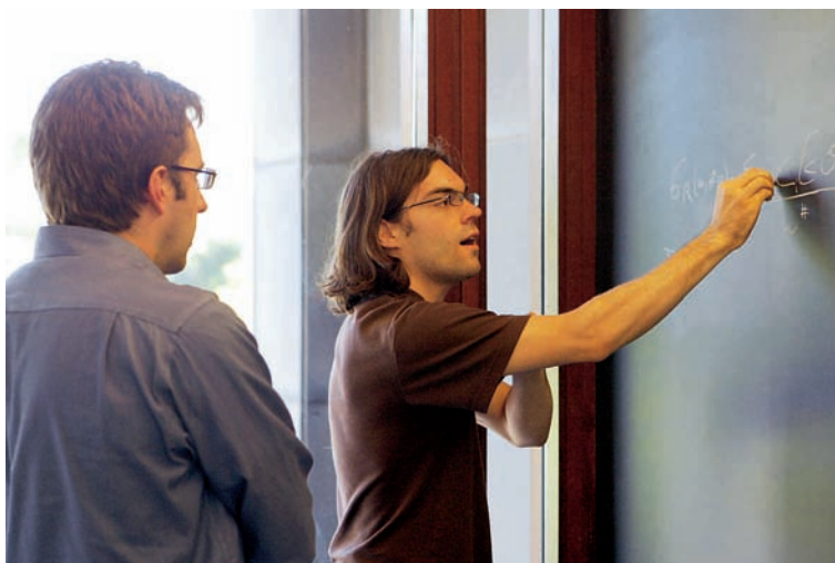
Member Simon Caron-Huot (right) studied very hot and dense systems such as the quark-gluon plasma and was also interested in gravitational, especially black hole, physics.
