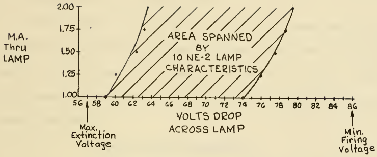
Figure 13. NE-2 Characteristics
