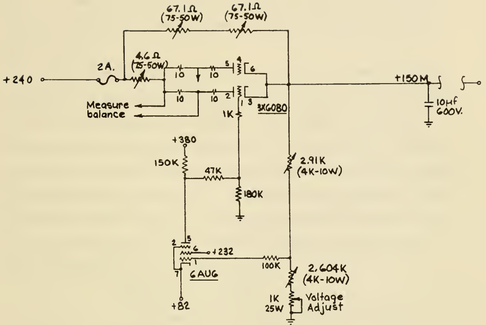
TYPICAL REGULATOR
