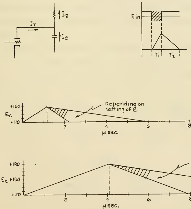
Figure 21. Operation of Stretcher Circuit
