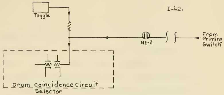
Figure 22. Graph Priming Circuit
